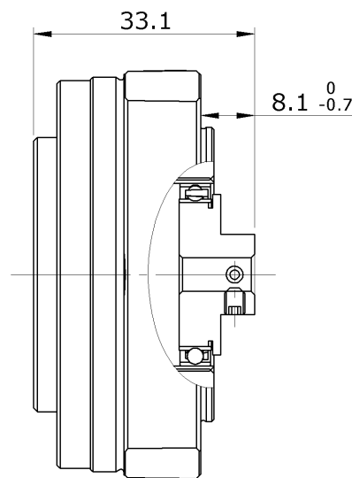
Dimension of interface at counter-assembly
